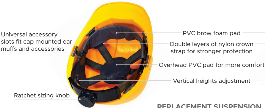
RS1404: 4-Point Ratchet Suspension
