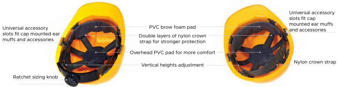
RS1404: 4-Point Ratchet Suspension
